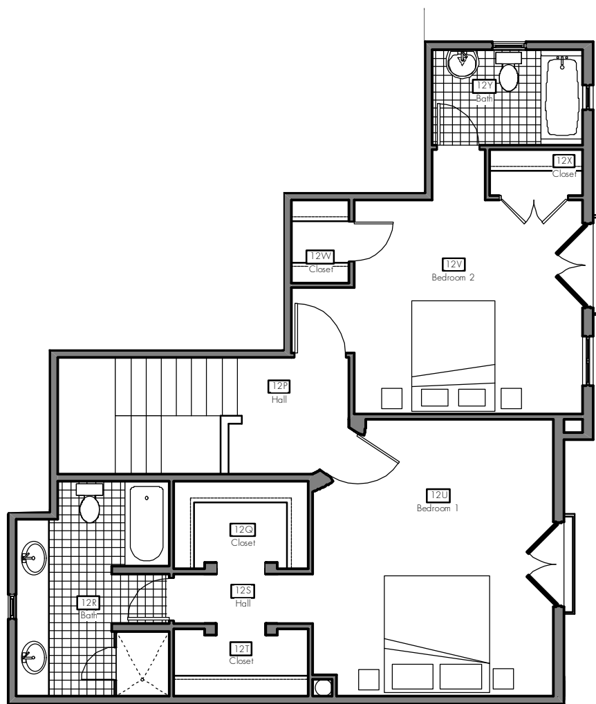
Third Floor - Unit 12 Upper Floor Plan Scale: 1/8" = 1'-0"
